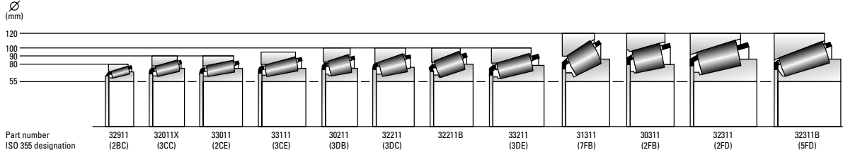
Comparison of ISO bearing designs (55 mm bore diameter)
