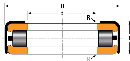
Fig. 80. Type TTSPS.
