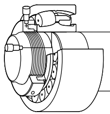
Fig. 52. Hydraulic nut used to mount the bearing on a tapered journal.
