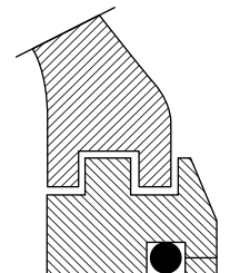
Fig. 28. Labyrinth seals.
