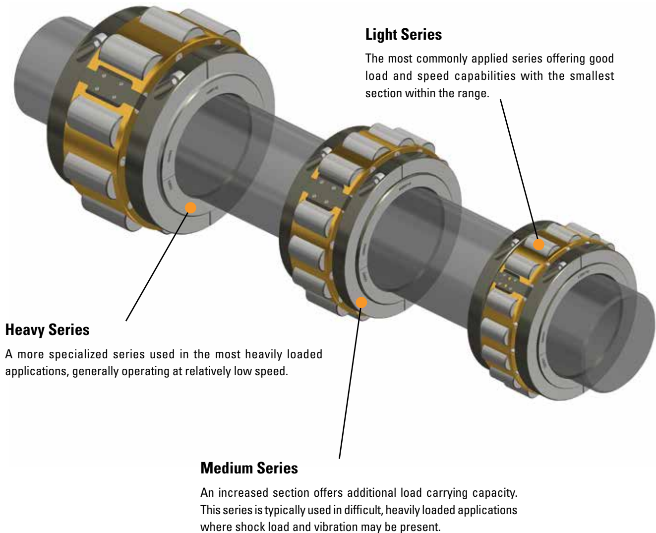
Fig. 10. Series comparison.
