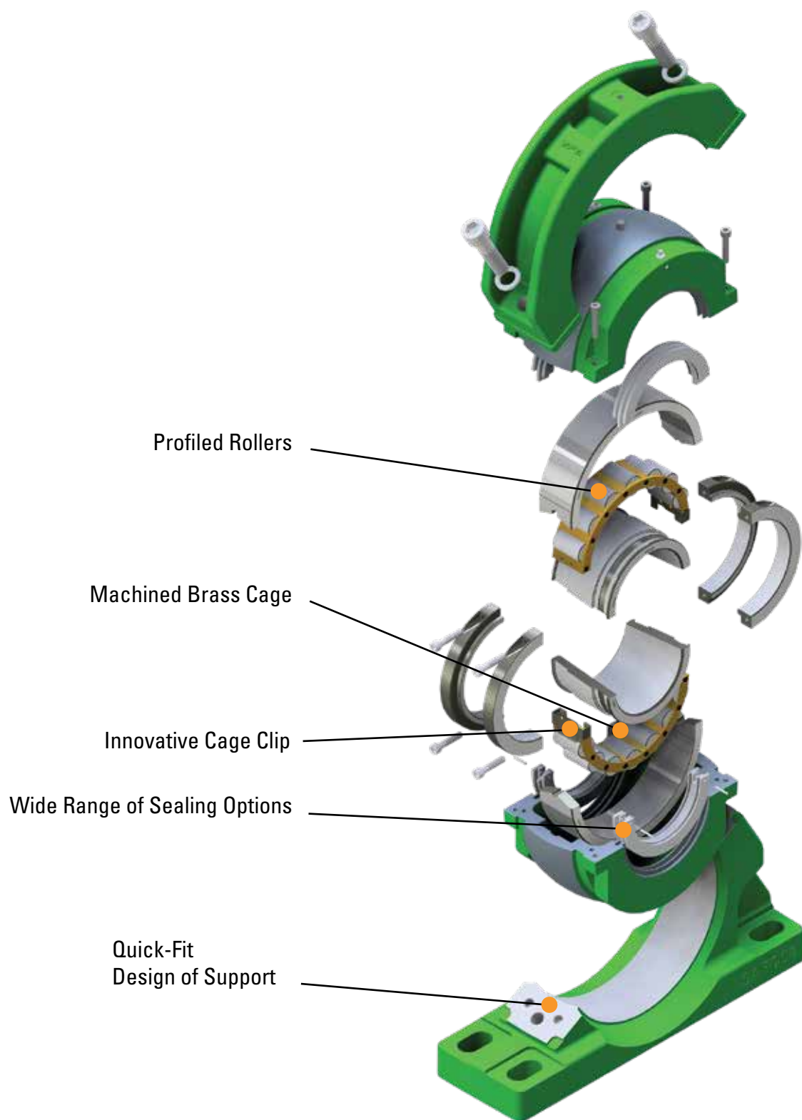
Fig. 2. Technical features.
