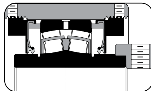
Fig. 15. Double-lip seals.
