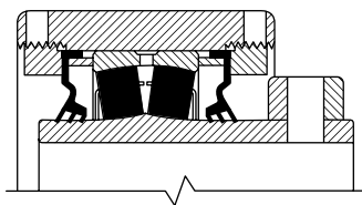
Fig. 9. Single set screw lock.
