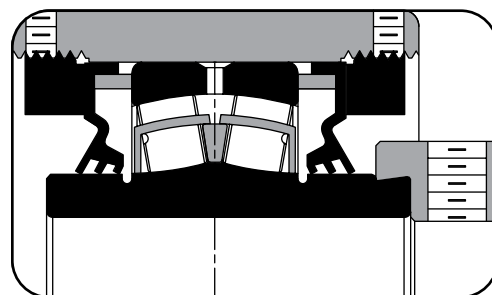
Fig. 13. Triple-lip seals.
