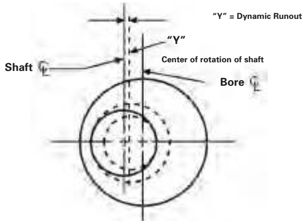
Figure 6 — Dynamic Runout
